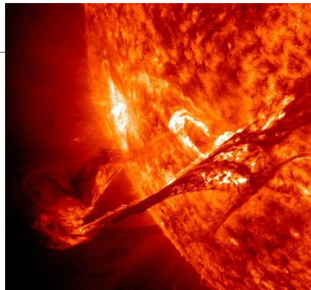
▲ Solar flares such as this one from August 2012 could wreak havoc on electromagnetic systems on Earth.
